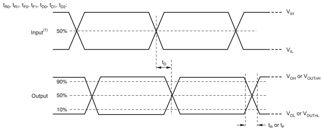
Figure 5. Output Timing
