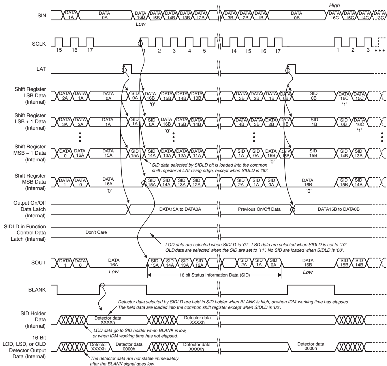
Figure 30. SID Read Timing
