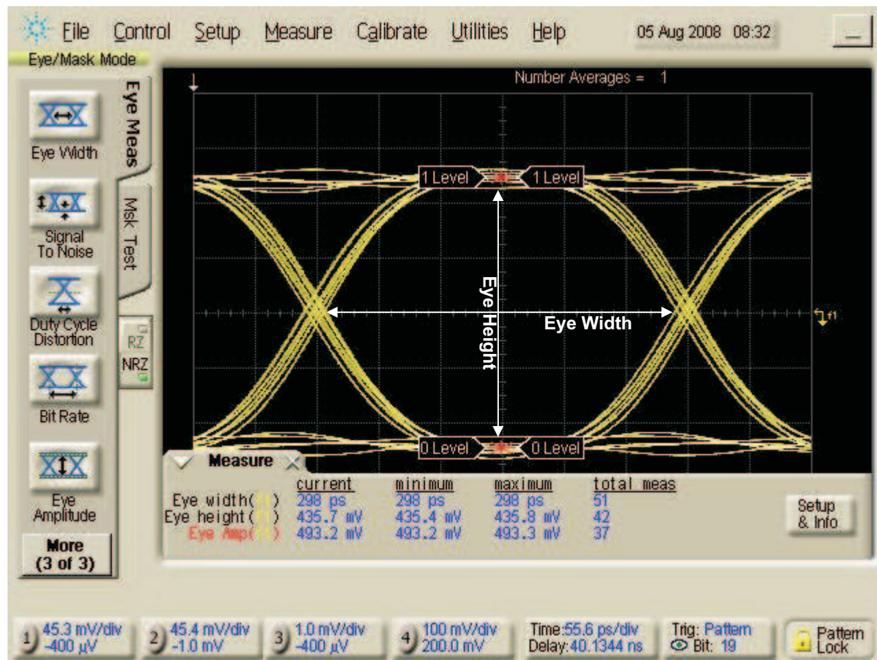
Figure 7. Eye Pattern
