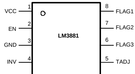
Figure 1. Top View VSSOP-8 Package
