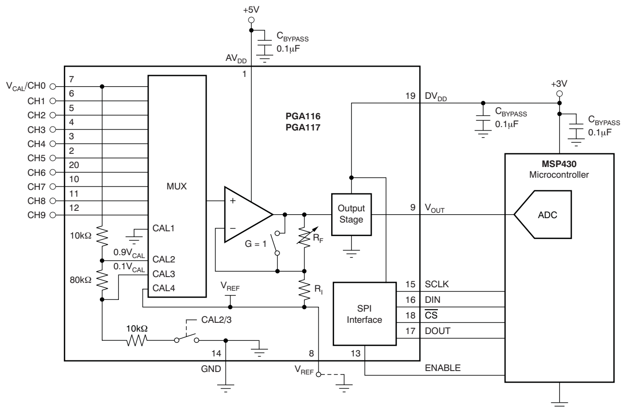
Figure 5. PGA116, PGA117 (TSSOP-20)
