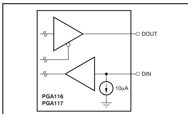
Figure 58. Digital I/O Structure—PGA116/PGA117
