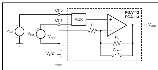
Figure 65. PGA112/PGA113 Configuration for Positive and Negative Excursions Around Midsupply Virtual Ground
