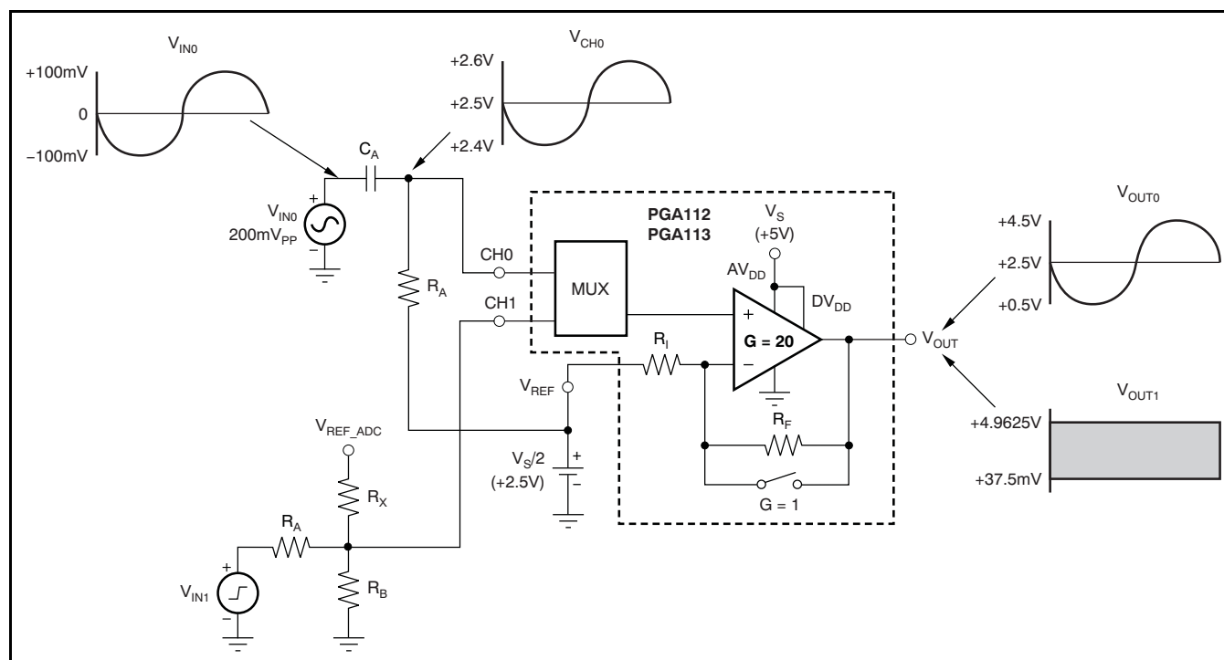
Figure 70. General-Purpose Input Scaling
