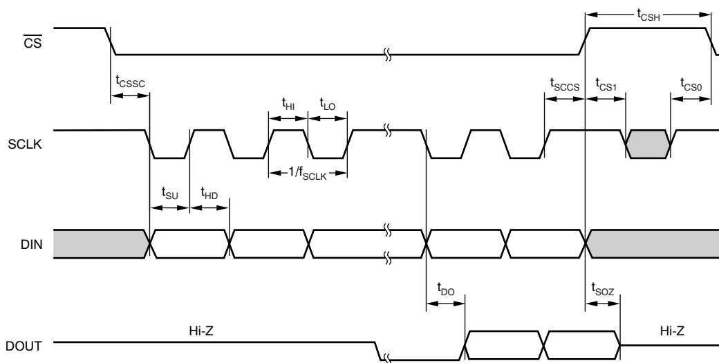
Figure 3. SPI Mode 1, 1
