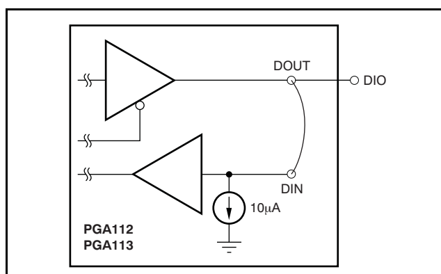
Figure 59. Digital I/O Structure—PGA112/PGA113
