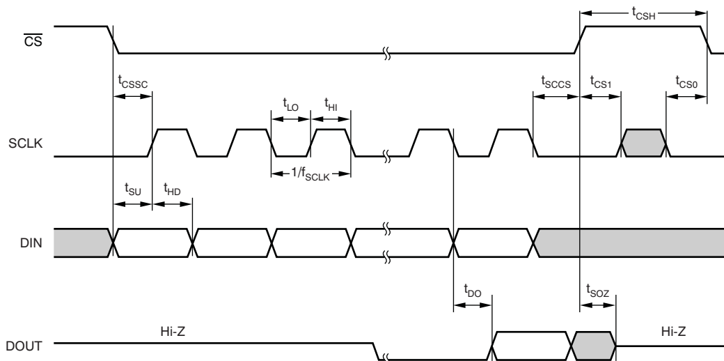
Figure 2. SPI Mode 0, 0
