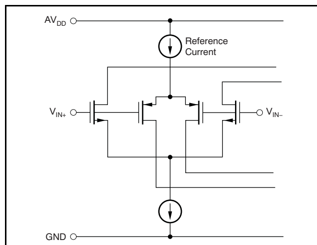
Figure 61. PGA Rail-to-Rail Input Stage
