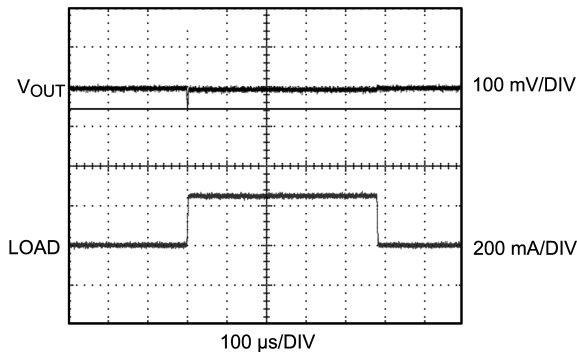
Load Transient Load = 0mA \leftrightarrow 250mA, 25^{\circ}C
