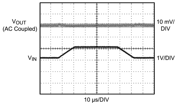
Line Transient V_{IN} = 3.2V \leftrightarrow 4.2V , Load = 250mA
