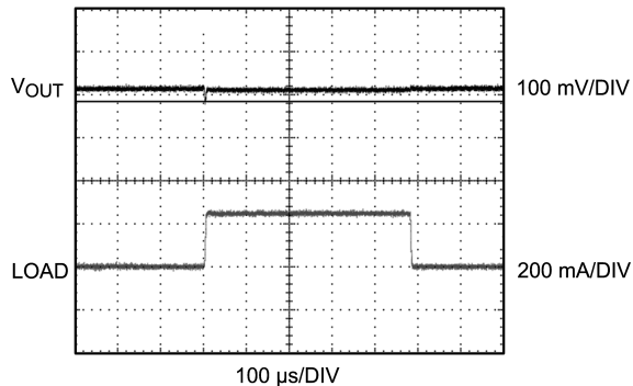
Load Transient Load = 0mA \leftrightarrow 250mA, -40^{\circ}C
