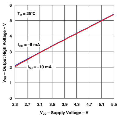
OUTPUT HIGH VOLTAGE VS SUPPLY VOLTAGE
