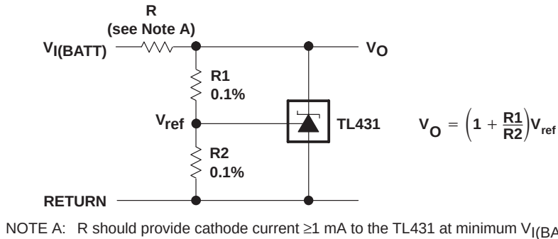
Figure 17. Shunt Regulator
