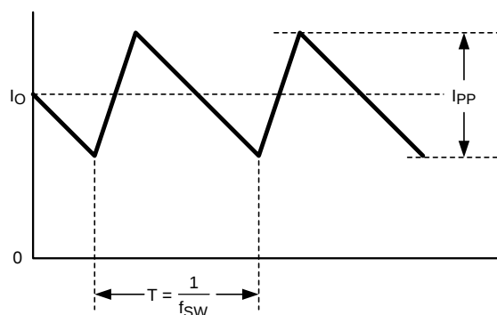
Figure 35. Inductor Current
