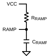
Figure 39. R_{\text{RAMP}} to VCC for V_{\text{OUT}} > 7.5\text{V}
