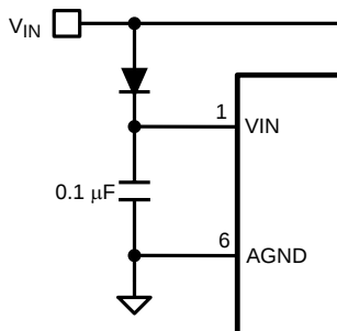
Figure 28. Input Blocking Diode for VCCX > VIN
