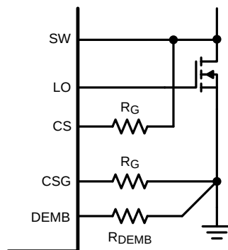
Figure 32. R_{DS(ON)} Current Sensing without Diode Emulation
