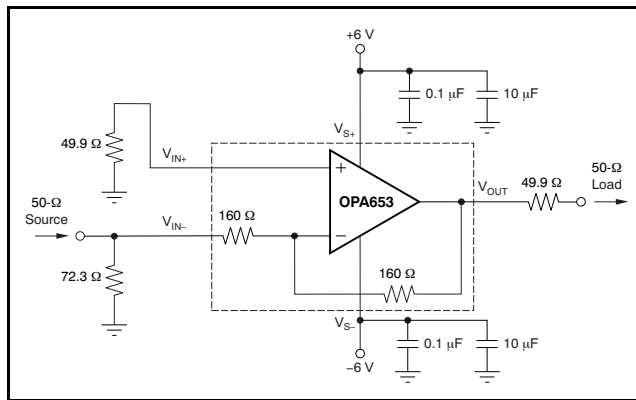
Figure 22. Noninverting Gain of -1 V/V in 50-Ω Test Environment
