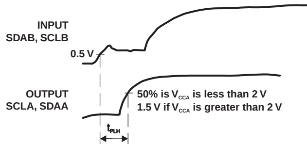
Figure 4. Waveform 3
