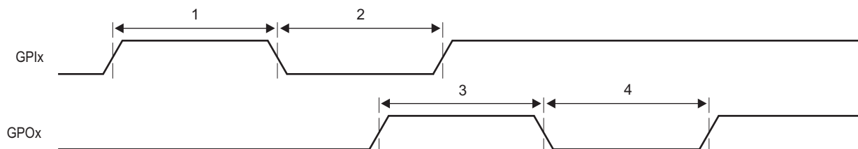
Figure 7-60 GPIO Timing
