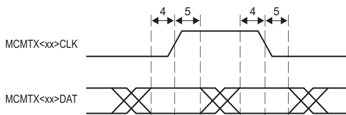
Figure 7-42 HyperLink Station Management Transmit Timing
