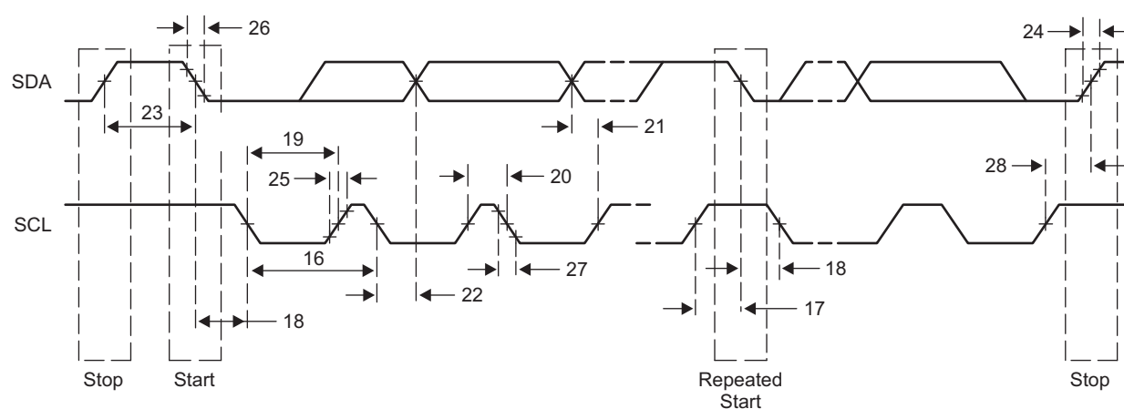
Figure 7-38 I 2 C Transmit Timings
