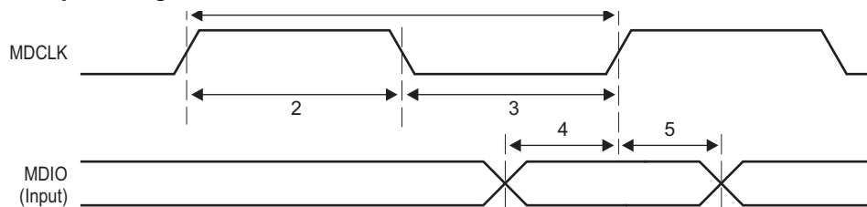
Figure 7-57 MDIO Input Timing
