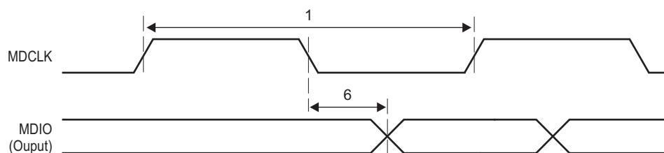
Figure 7-58 MDIO Output Timing
