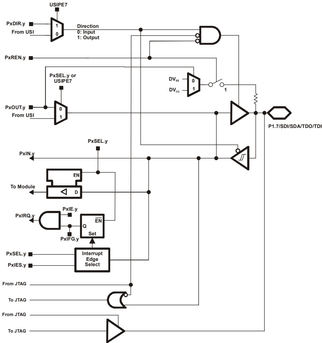
Port P1 (P1.7) pin functions - MSP430G2x21
