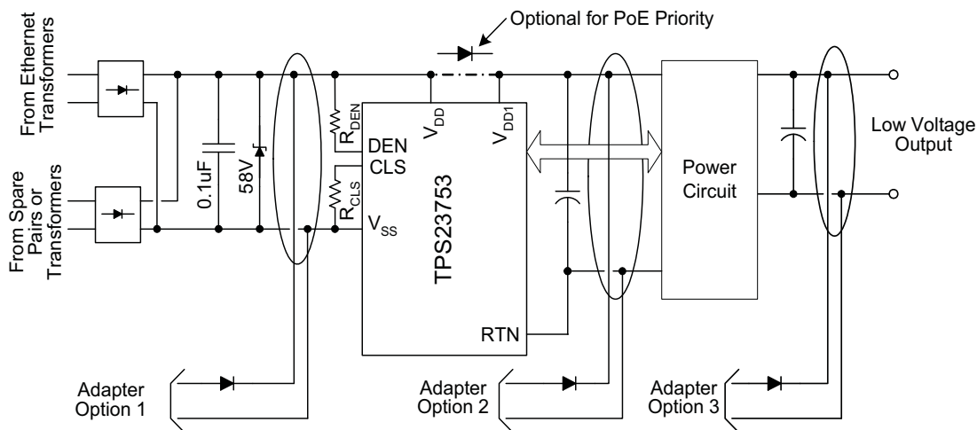
Figure 24. ORing Configurations
