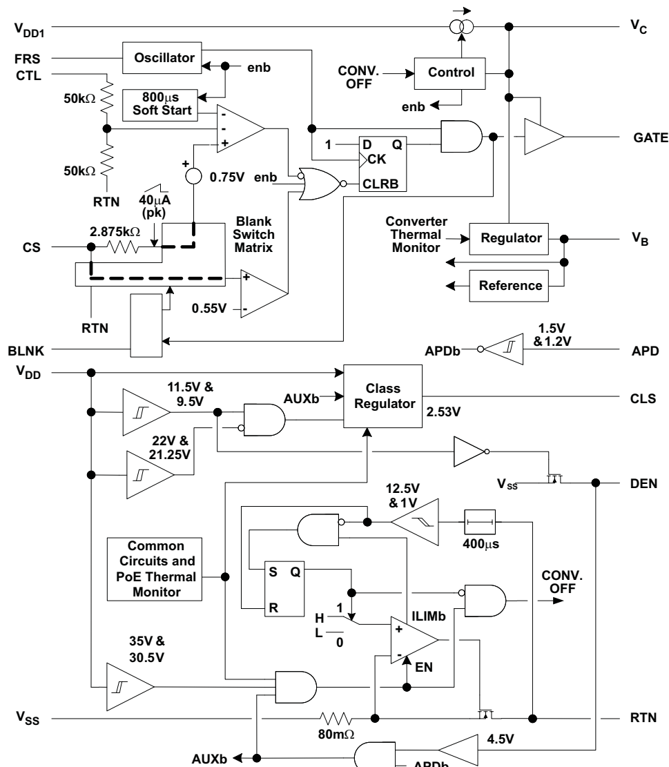
Figure 2. TPS23753A Functional Block Diagram
