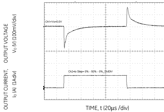
Figure 34. Transient Response to Dynamic Load Change from 0% to 50% to 0%.
