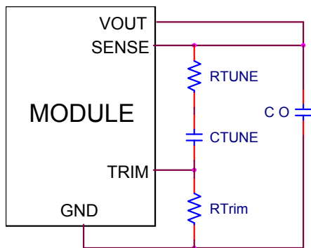
Figure 58. Circuit diagram showing connection of R_{TUNE} and C_{TUNE} to tune the control loop of the module.
