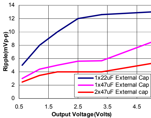
Figure 52. Output ripple voltage for various output voltages with external 1x22 µF, 1x47 µF or 2x47 µF ceramic capacitors at the output (2A load). Input voltage is 12V.
