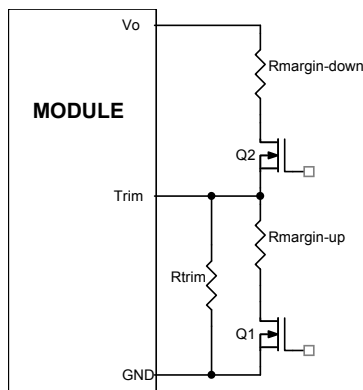
Figure 57. Circuit Configuration for margining Output voltage.
