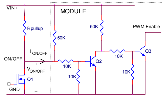
Figure 53. Circuit configuration for using positive On/Off logic.
