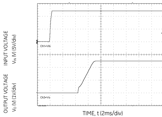
Figure 24. Typical Start-up Using Input Voltage ( V_{in} = 12V , C_{ext}= 22\mu F , I_o = I_{o,max} ).
