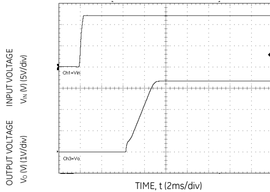
Figure 30. Typical Start-up Using Input Voltage ( V_{IN} = 12V , C_{ext}= 22\mu F , I_o = I_{o,max} ).
