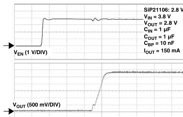
20 µs/DIV Output Voltage Start-Up
