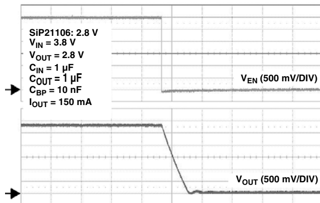
20 µs/DIV Output Voltage Power-Down
