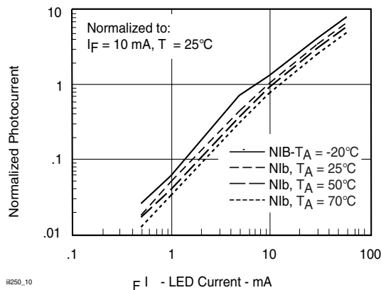
Fig. 10 Normalized Photocurrent vs. I_F and Temp.
