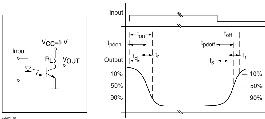
Figure 8. Switching Test Circuit
