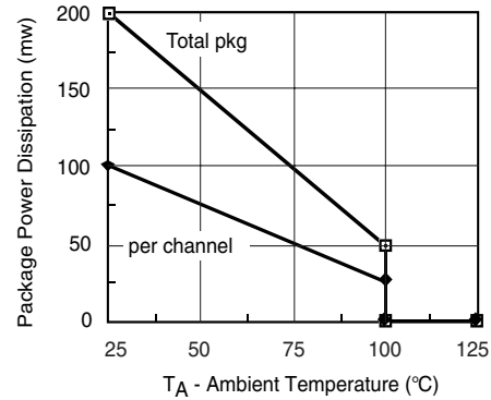
Figure 7. Power Dissipation vs. Ambient Temperature
