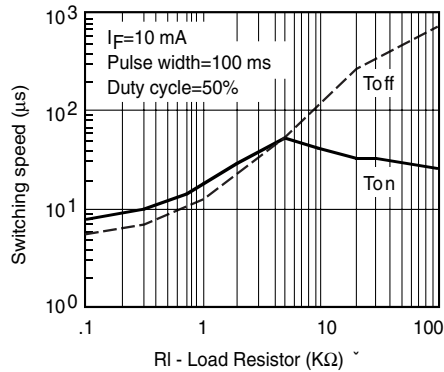
Figure 5. Switching Speed vs. Load Resistor
