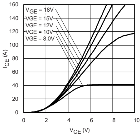
Fig. 7 - Typical IGBT Output Characteristics T J = 125 °C; t p = 80 μs
