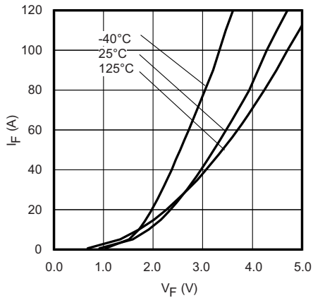
Fig. 8 - Typical Diode Forward Characteristics t p = 80 μs
