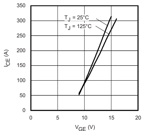
Fig. 12 - Typical Transfer Characteristics V CE = 50 V; t p = 10 μs
