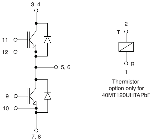
Fig. 25 - Electrical diagram
