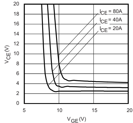
Fig. 11 - Typical V CE vs. V GE T J = 125 °C
