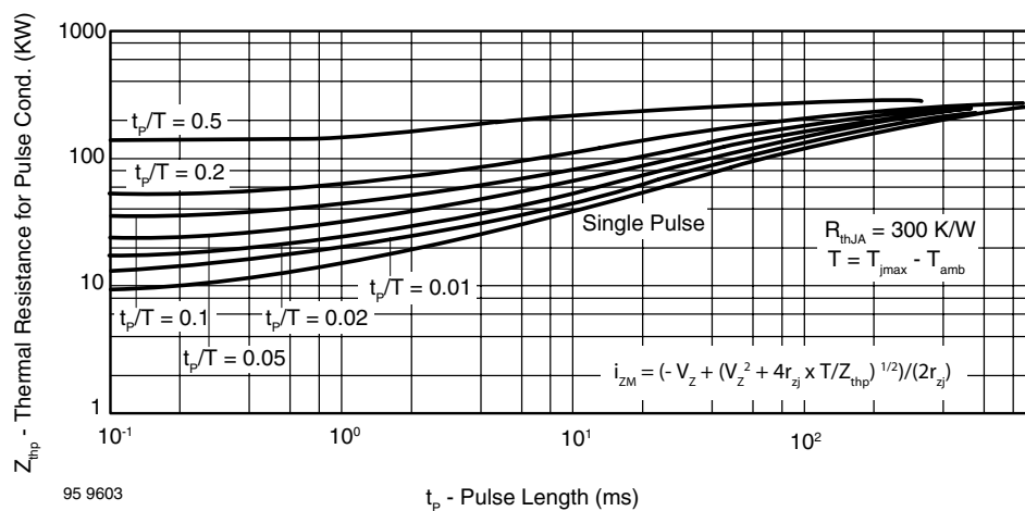
Figure 11. Thermal Response
