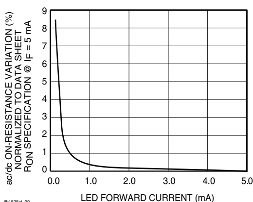
Figure 10. Variation in ON-Resistance vs. LED Current
