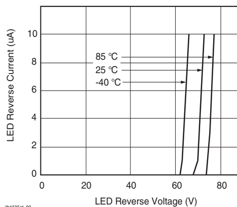
Figure 4. LED Reverse Current vs. LED Reverse Voltage
