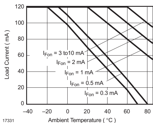
Figure 1. Recommended Operating Conditions
