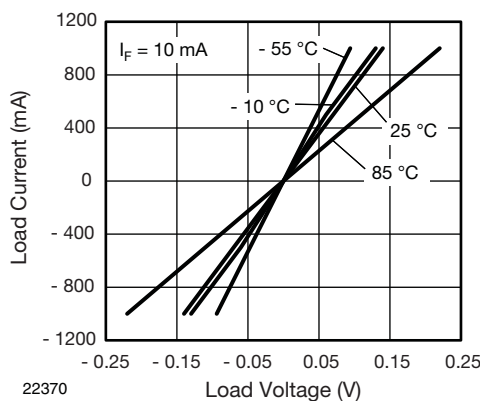
Fig. 13 - Load Current vs. Load Voltage
