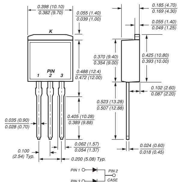
TO-262AA (MBRB30H150CT-1)
