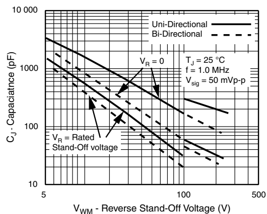
Figure 6. Capacitance
