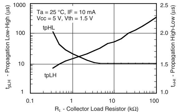
Fig. 12 - Propagation Delay vs. Collector Load Resistor
