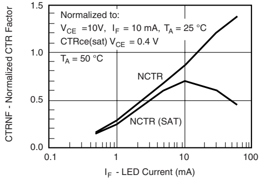
Fig. 7 - Normalized Non-Saturated and Saturated CTR vs. LED Current
