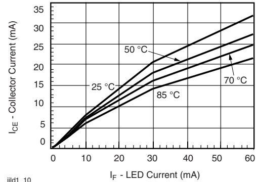
Fig. 10 - Collector Emitter Current vs. Temperature and LED Current
