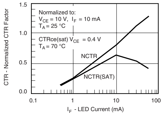
Fig. 8 - Normalized Non-Saturated and Saturated CTR vs. LED Current
