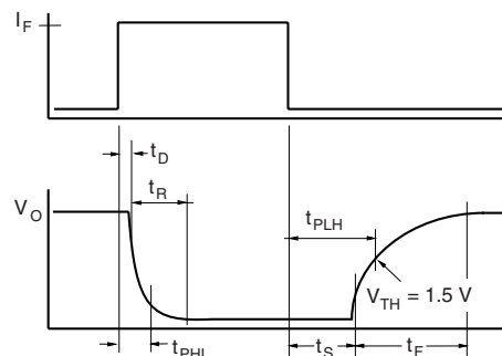
Fig. 4 - Saturated Switching Timing
