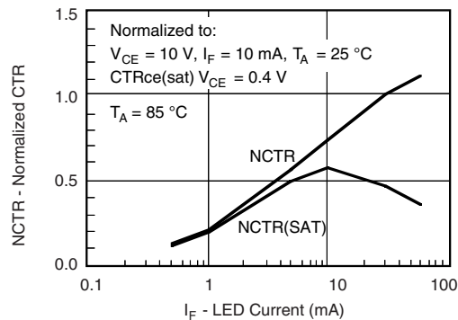
Fig. 9 - Normalized Non-Saturated and Saturated CTR vs. LED Current
