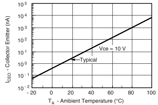
Fig. 11 - Collector Emitter Leakage Current vs. Temperature
