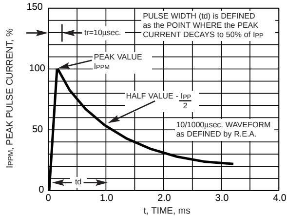
FIG. 3 - PULSE WAVEFORM
