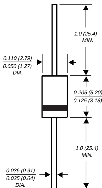
DO-204AM
