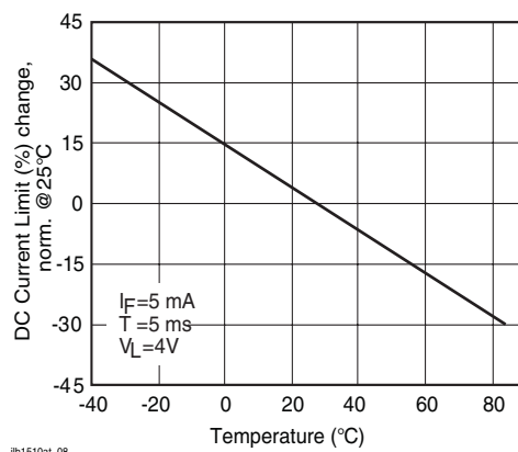
Figure 9. DC Current Limit vs. Temperature
