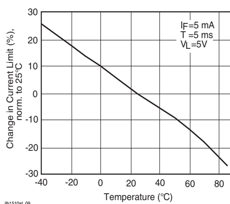
Figure 10. Current Limit vs. Temperature
