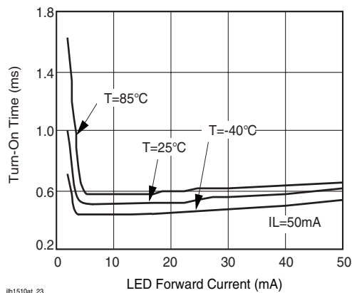
Figure 24. Turn-on Time vs. LED Current
